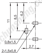
PCB LAYOUT (TOP VIEW)
